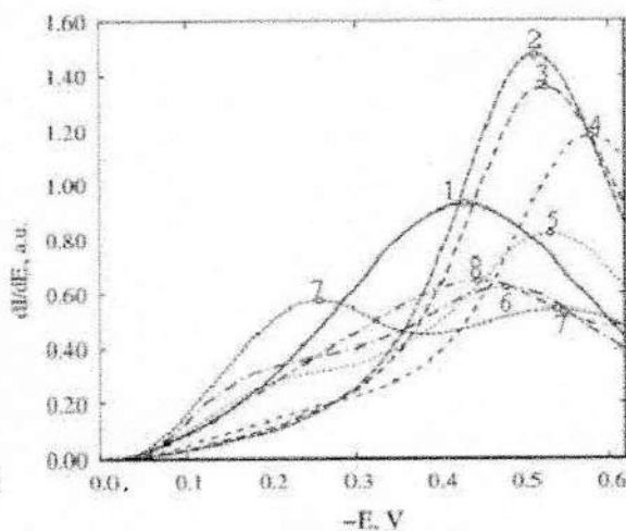
Figure 6. The differential voltammograms for the oxygen reduction on platinum in the background electrolyte 0,1 M NaCl in water (1), containing the ions \text{Fe}^{2+} (2 - 2,42), with the different concentrations of 2i: 3 - 0,09; 4 - 0,20; 5 - 0,38; 6 - 0,57; 7 - 0,74; 8 - 0,91 mM.
