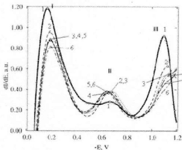
Figure 7. Differential voltammograms of oxygen reduction on copper in the presence of different concentrations (2-6) of 3c:
