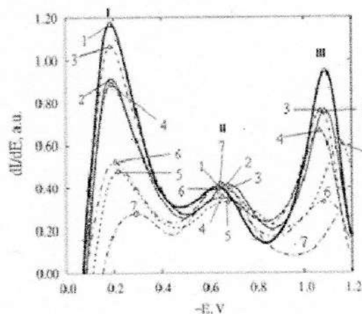
Figure 3. The differential voltammogram of the oxygen reduction on copper in the presence of different concentrations (2-6) of the compound 1i: 1 - background 0,1 M NaCl; 2 - 0,2; 3 - 0,38; 4 - 0,57; 5 - 0,74; 6 - 0,90; 7 - 1,07 mM.
